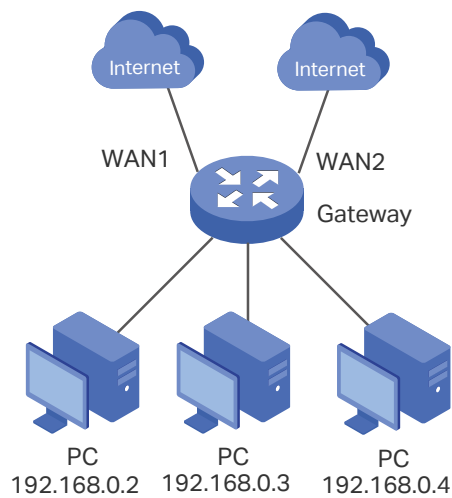
Figure 8-9 Network Topology
